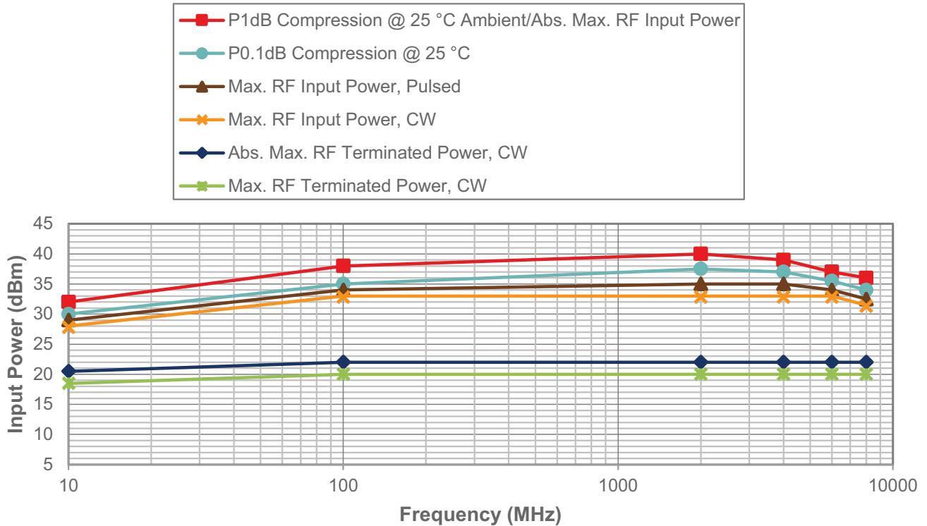
Figure 2 ▪ Power De-rating Curve, 10 MHz–8 GHz, –40 °C to +105 °C Ambient, 50?
