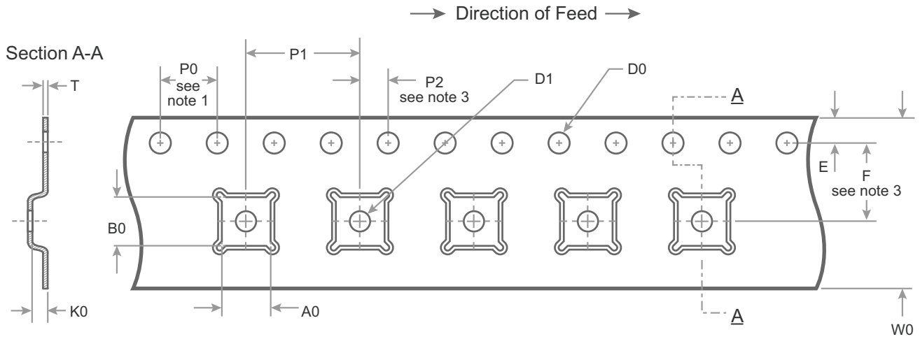
Figure 25 - Tape and Reel Specifications for 24-lead 4 x 4 x 0.85 mm QFN
