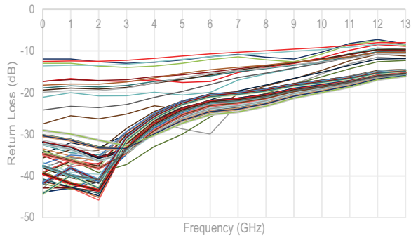
Figure 14 ■ Input Return Loss (All Attenuation States)
