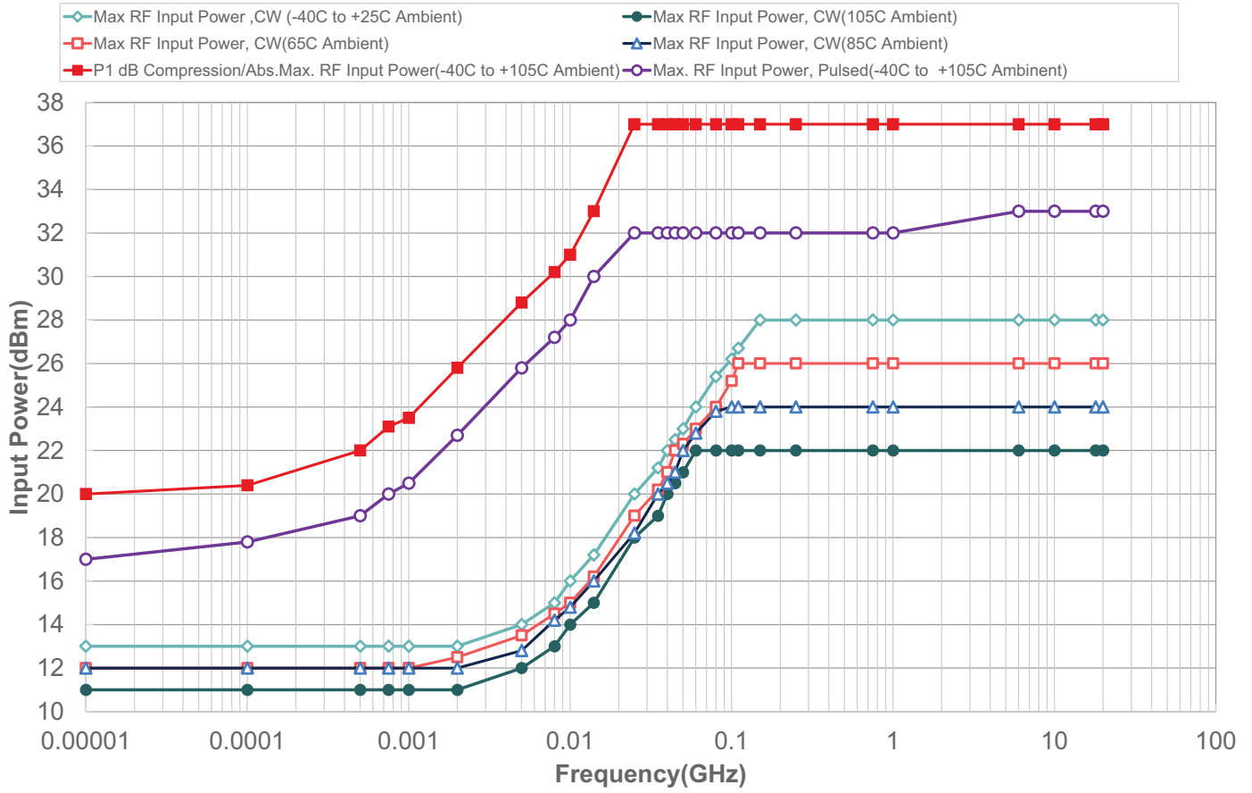
Figure 7 ■ Power De-rating Curve, 9 kHz–55 GHz, 50 Ohm
