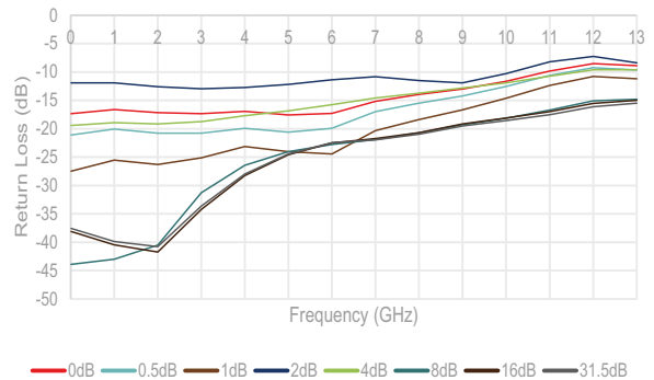
Figure 13 ■ Input Return Loss (Major Attenuation States)
