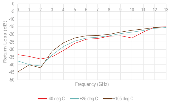
Figure 12 ■ Output Return Loss (Ref State) vs. Temperature
