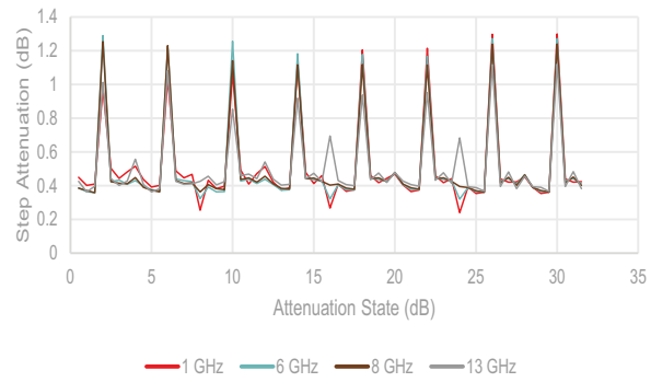
Figure 25 ■ 0.5 dB Step Actual vs. Frequency
