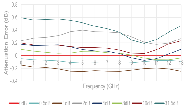
Figure 27 ■ 0.5 dB Major State Bit Error vs. Attenuation State
