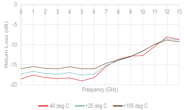
Figure 11 ■ Output Return Loss (Ref State) vs. Temperature
