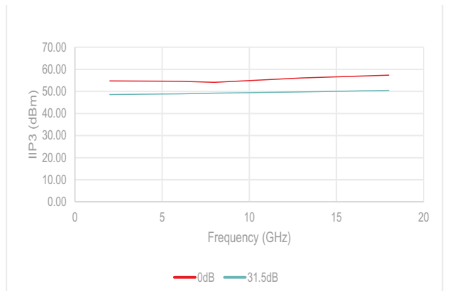
Figure 33 ■ IIP3
