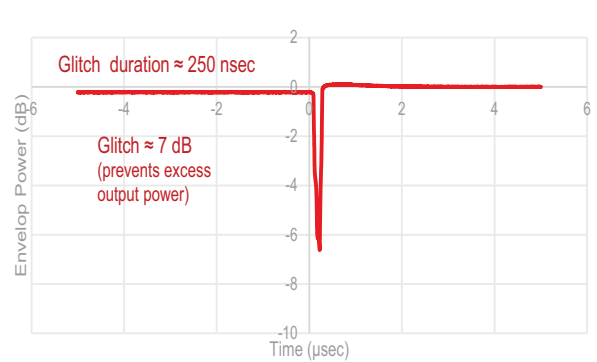
Figure 31 ■ Attenuation Transient (24 dB to 23.5 dB)
