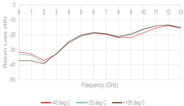
Figure 12 ■ Output Return Loss (Ref State) vs. Temperature
